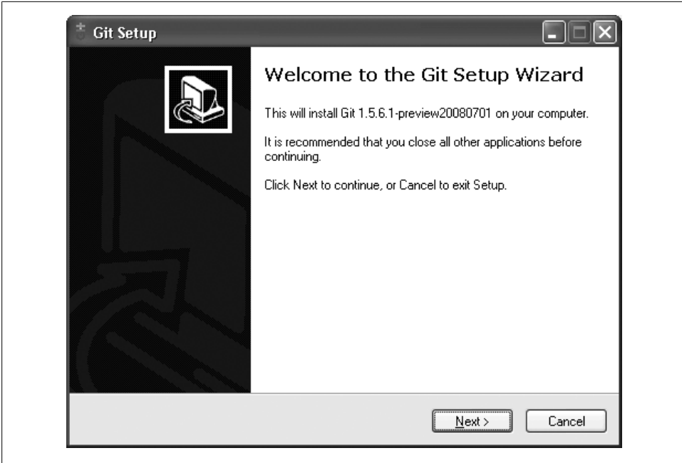
Figure 2-3. msysGit setup
